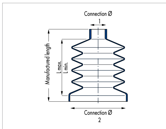
Drawing with dimensions multiple convolution bellows
