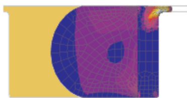
Figure 01: PTFE back-up ring at 40 MPa
