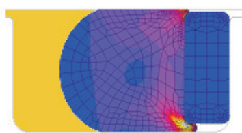
Figure 02: PA back-up ring at 20 MPa
