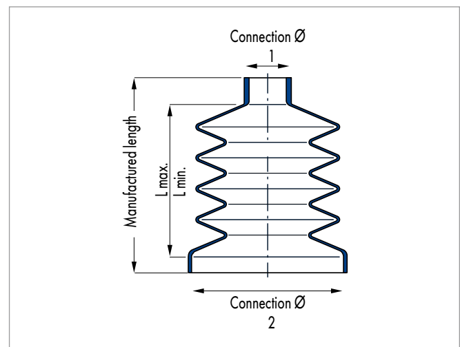
Drawing with dimensions multiple convolution bellows
